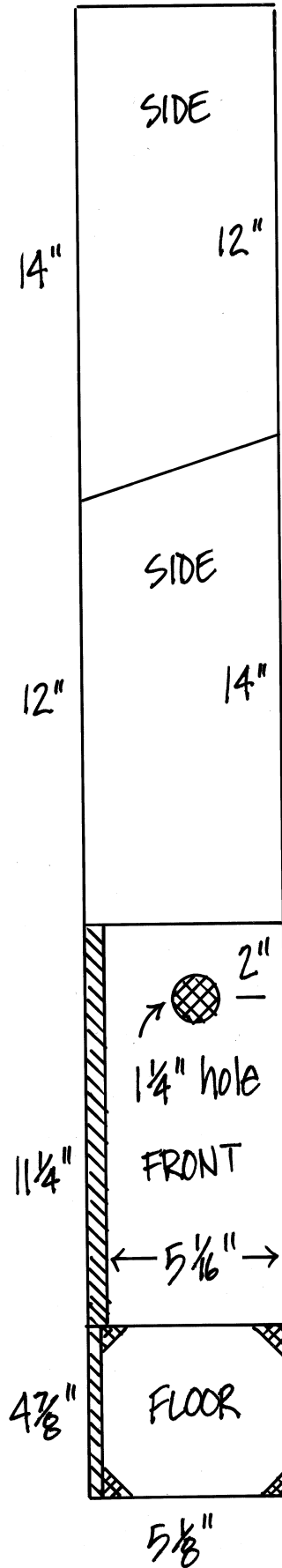
Sunset Magazine Birdhouse Cutting Diagram
